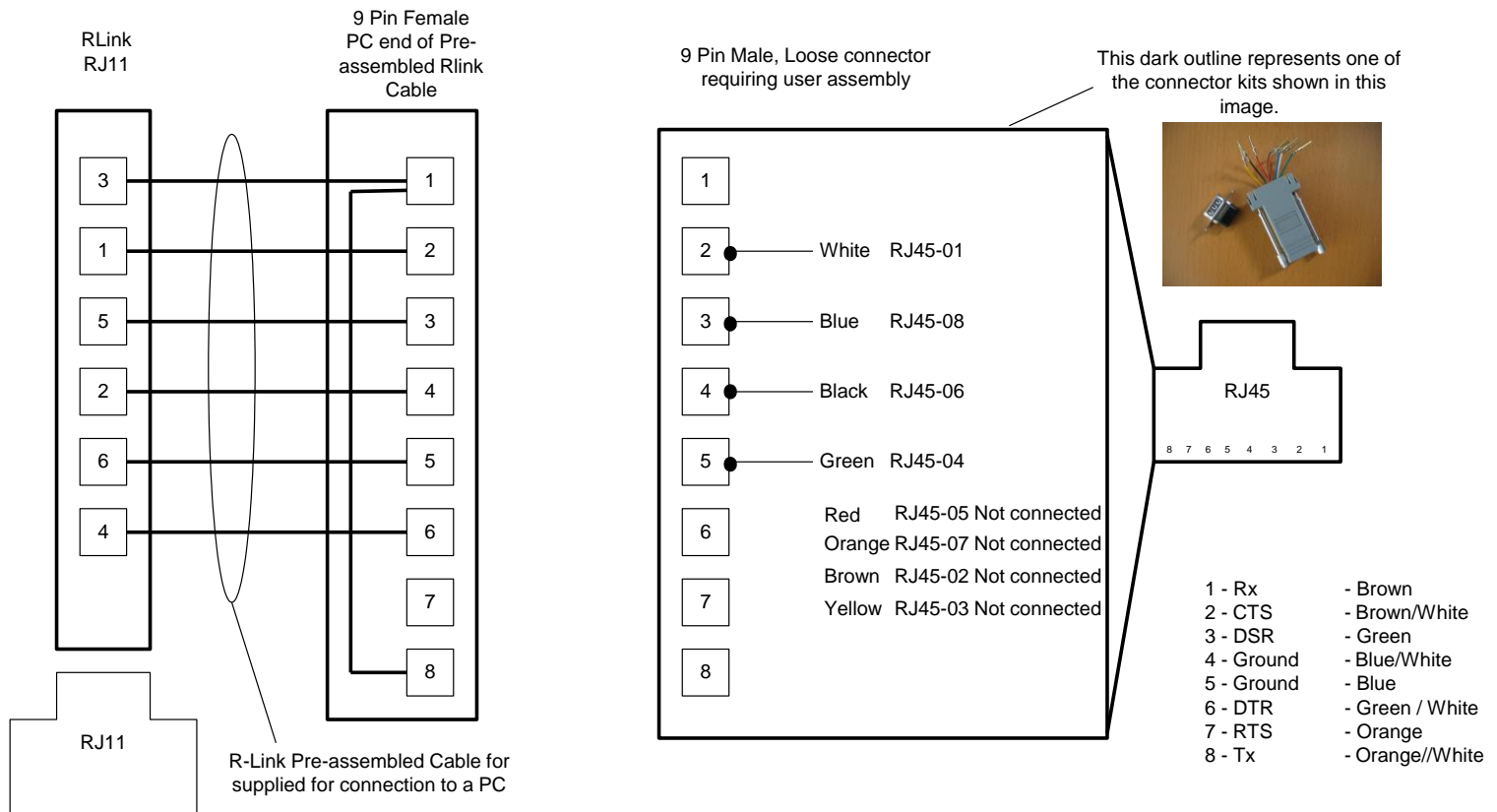
GE-TLC Rlink to FieldServer using pre-assembled GE-TLC Rlink-PC Cable.
