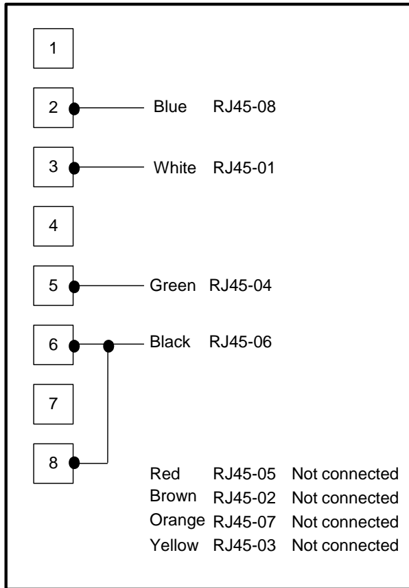
Tunnel Cable GE-TLC Configuration PC to FieldServer 's TLC Driver secondary port for FS20's and FS40's
